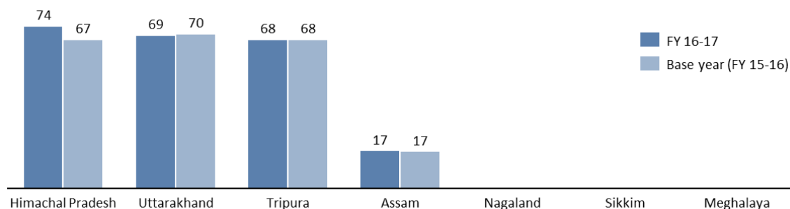
Figure 57: Indicator 9: The length of the canal and distribution network lined as on the end of the given FY vis-à-vis the total length of canal and distribution network found suitable (selected) for lining for improving conveyance efficiency—North-Eastern and Himalayan states
